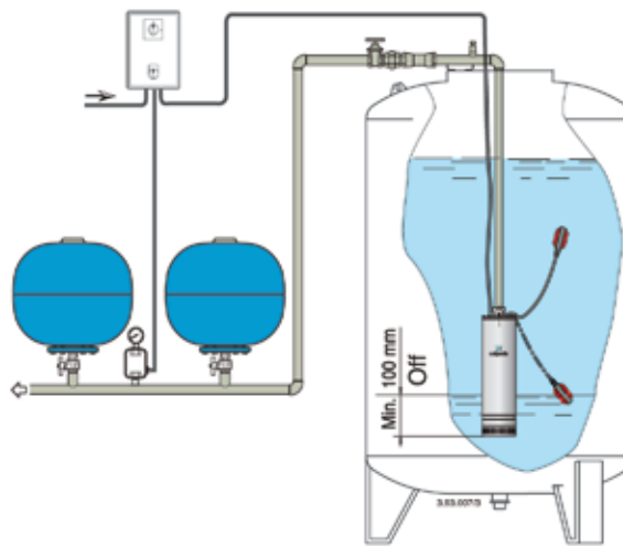
Installation example
